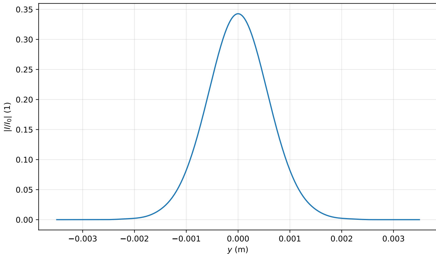
Intensity profile I(x=0, y, z=3.503)/I_0 , P_{in}=0.3P_{cr} , artificial time
